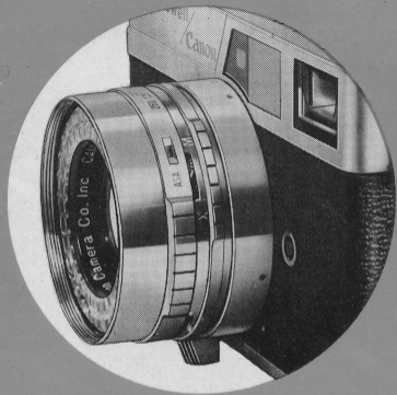
Set Flash-Setting Lever for Type of Bulb
